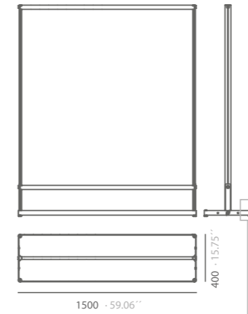
INL15PF adjustable feet · pies regulables
