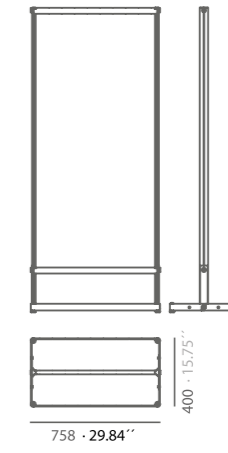
INL7PF / INL15PF adjustable feet · pies regulables
