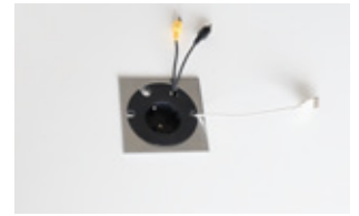
Socket + round 80mm grommet cover for tabletop: Manufactured in Zamak alloy and finished in matt chrome. The socket and grommet body is made of black plastic. The drill hole in the cover to facilitate insertion must be done by the customer.
